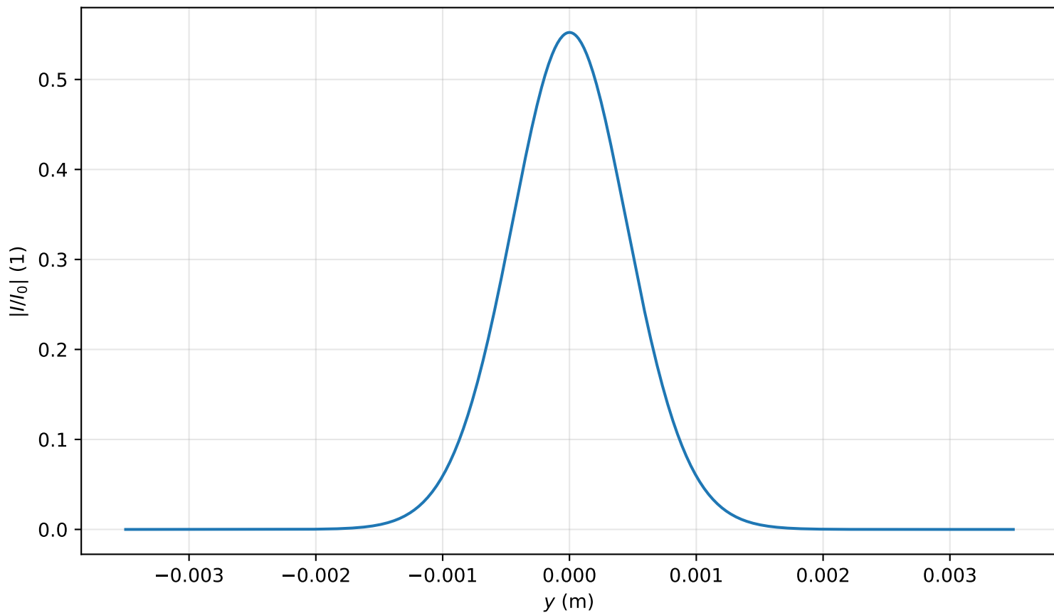
Intensity profile I(x=0, y, z=2.149)/I_0 , P_{in}=0.2P_{cr} , artificial time
